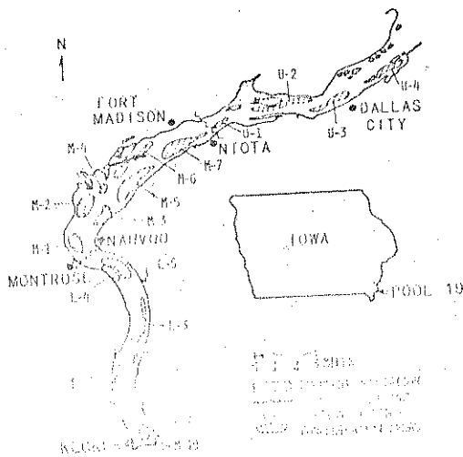
Fig. 1. Keokuk Pool study area from Keokuk, Iowa to Dallas City, Illinois. Three subdivisions are separated by jagged lines and concentration areas are indicated by section: lower (L), middle (M), and upper (U).
